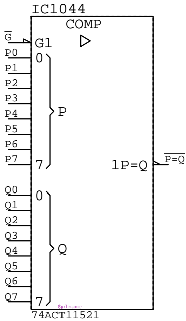
74ACT11521 IC????
