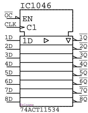
74ACT11534 IC????
