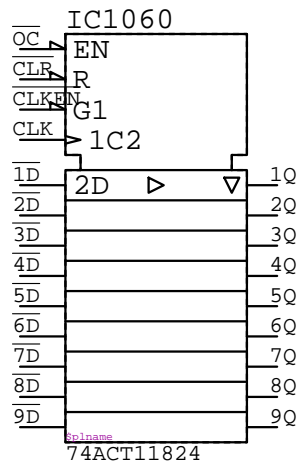
74ACT11824 IC?????
