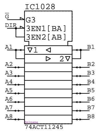
74ACT11245 IC?????
