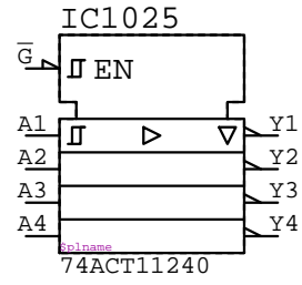
74ACT11240 IC?????
