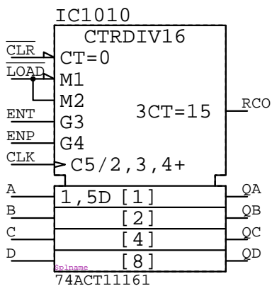
74ACT11161
