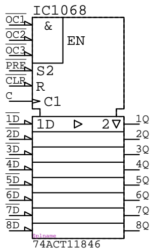
74ACT11846 IC?????
