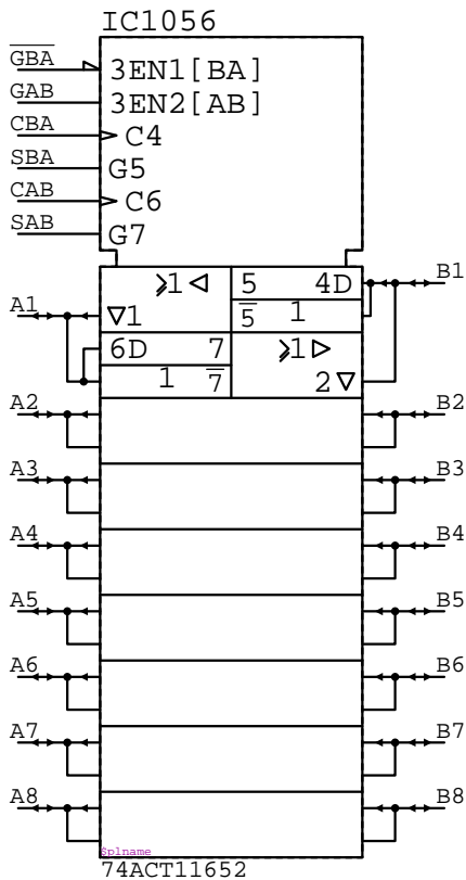
74ACT11652 IC?????
