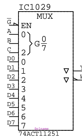
74ACT11251 IC?????
