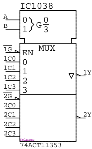
74ACT11353 IC????
