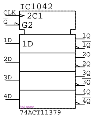
74ACT11379 IC????
