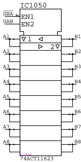
74ACT11623 IC?????
