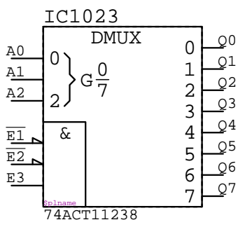
74ACT11238 IC?????
