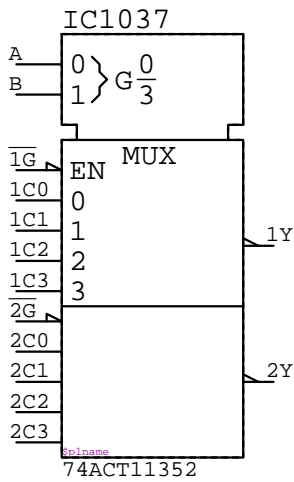
74ACT11352 IC????
