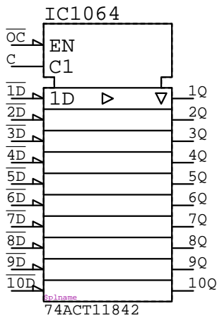
74ACT11842 IC?????
