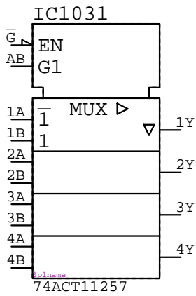
74ACT11257 IC?????
