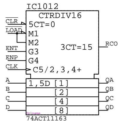
74ACT11163
