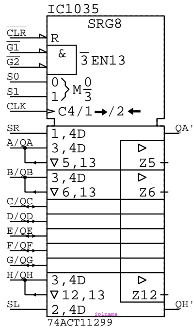
74ACT11299 IC?????
