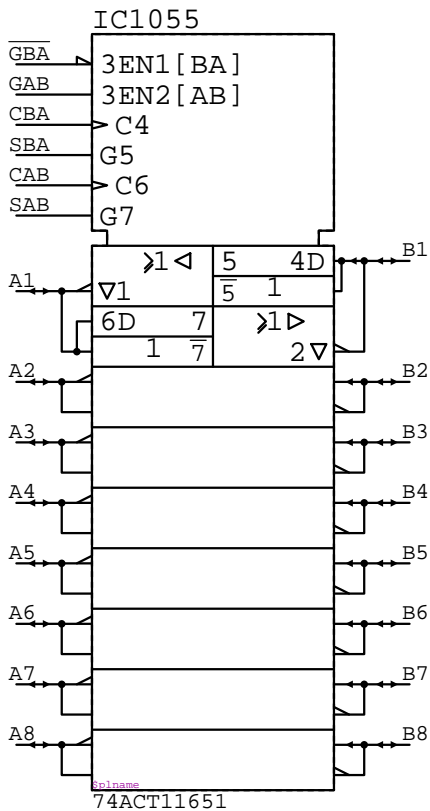
74ACT11651 IC?????
