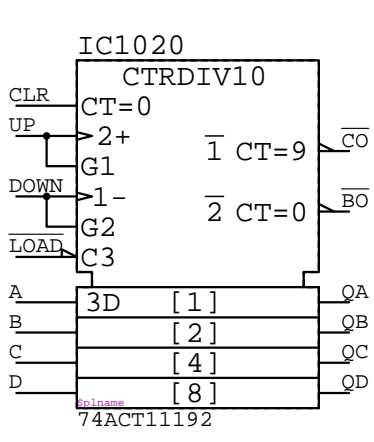
74ACT11192 IC?????
