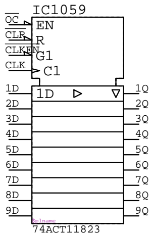
74ACT11823 IC?????
