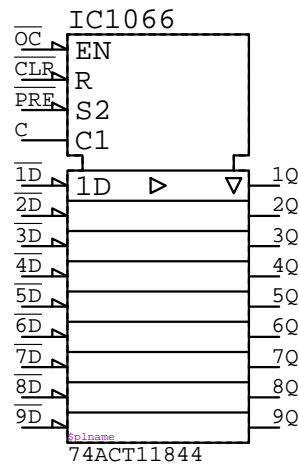
74ACT11844 IC?????
