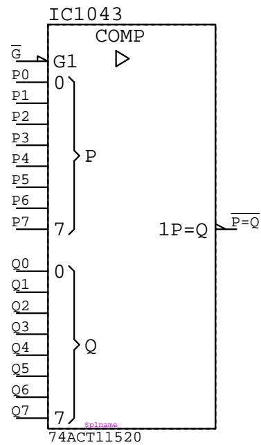
74ACT11520 IC????
