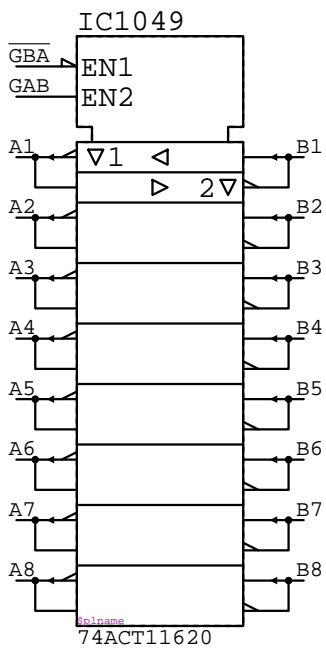
74ACT11620 IC?????
