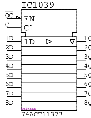
74ACT11373 IC????
