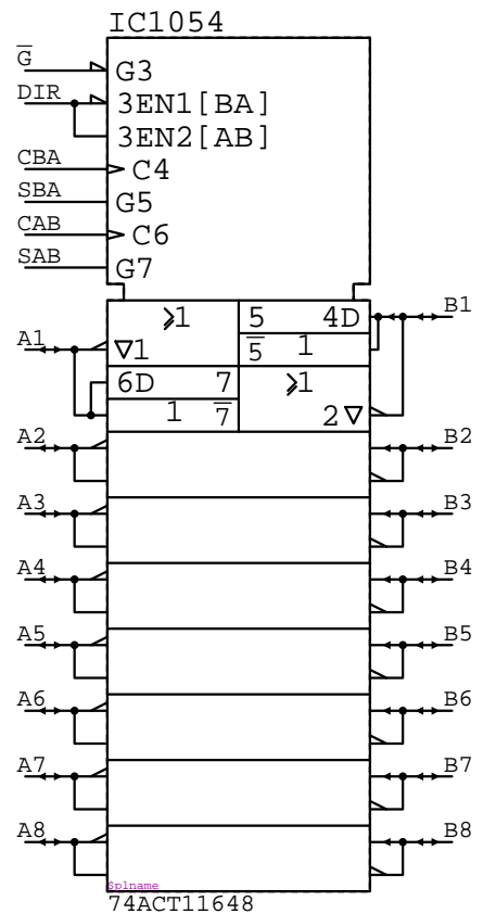
74ACT11648 IC?????
