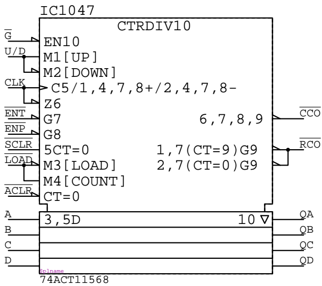
74ACT11568 IC????
