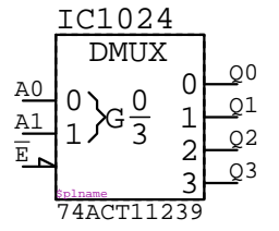
74ACT11239 IC?????
