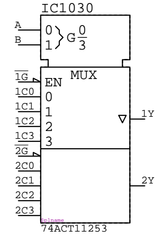
74ACT11253 IC?????
