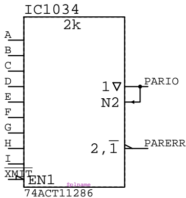
74ACT11286 IC?????
