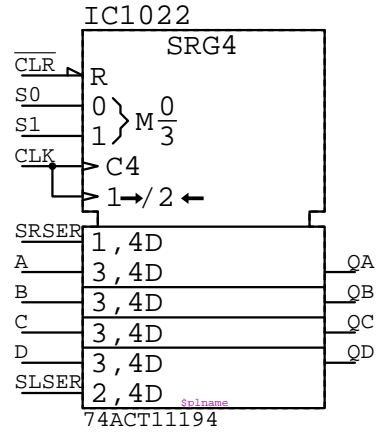
74ACT11194 IC?????
