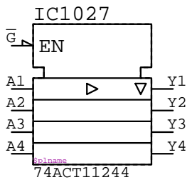
74ACT11244 IC?????
