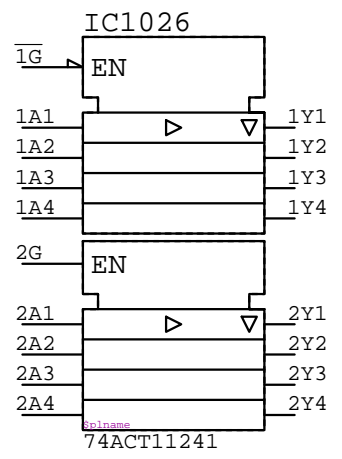
74ACT11241 IC?????
