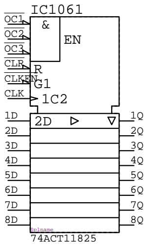
74ACT11825 IC?????
