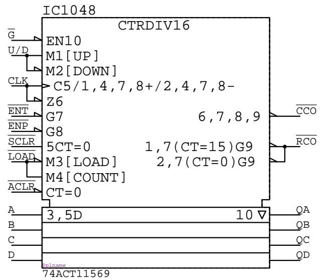
74ACT11569 IC????
