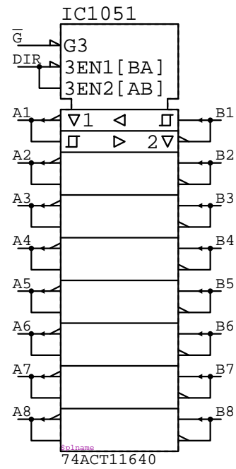
74ACT11640 IC?????
