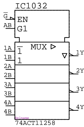
74ACT11258 IC?????
