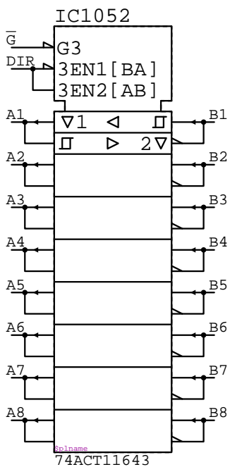
74ACT11643 IC?????
